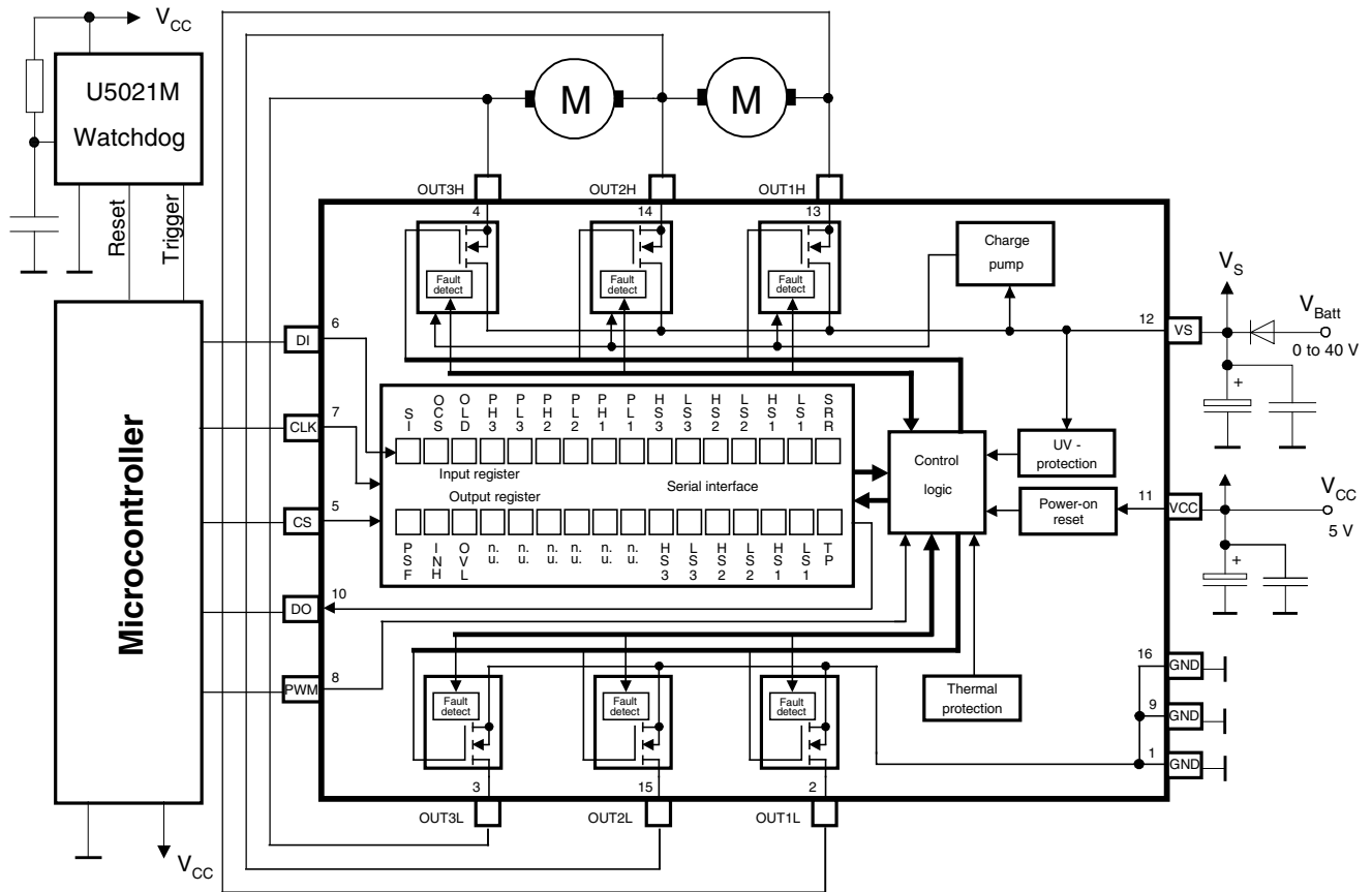
Figure 10-1. Application Circuit
