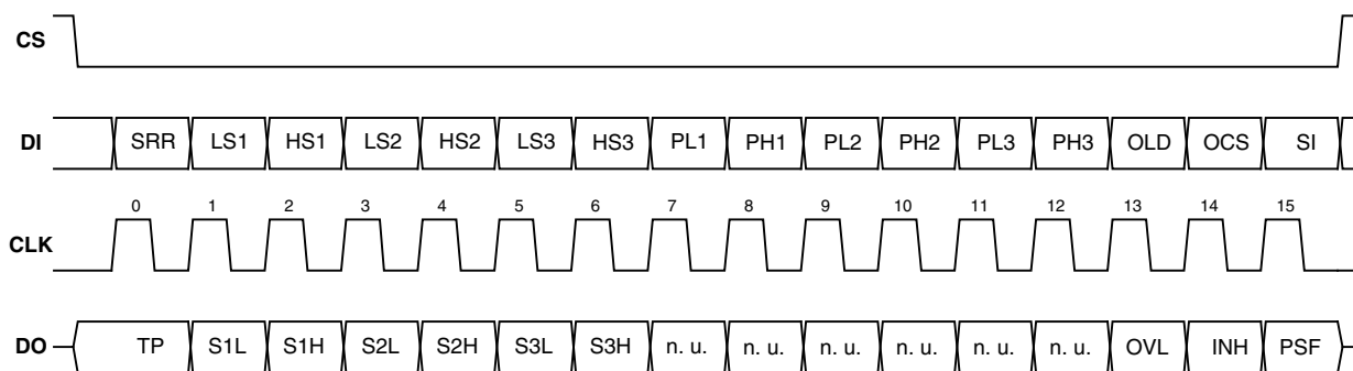
Figure 3-1. Data Transfer
